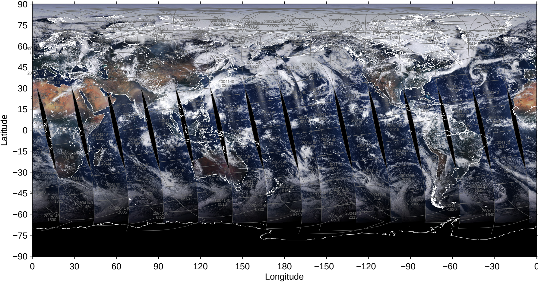
File = 200405/MYD02SSH-A2004140-pbin-005.1440-0721, RGB=645, 555, 469nm
