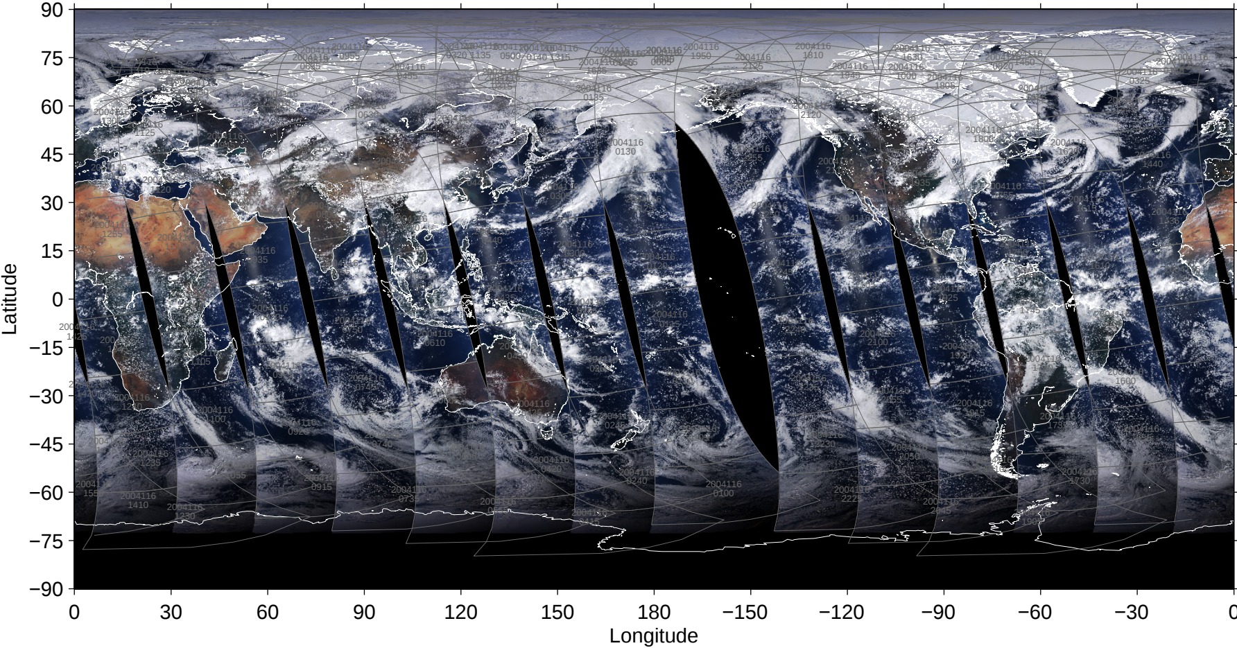
File = 200404/MYD02SSH-A2004116-pbin-005.1440-0721, RGB=645, 555, 469nm
