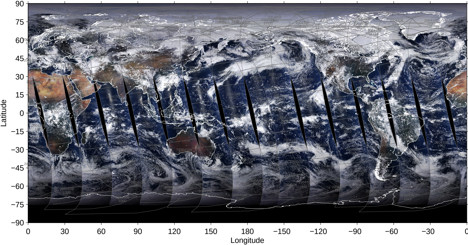
File = 200404/MYD02SSH-A2004108-pbin-005.1440-0721, RGB=645, 555, 469nm
