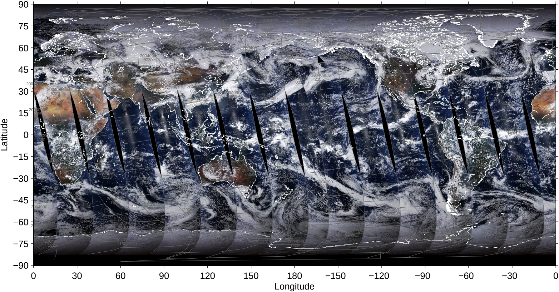
File = 200403/MYD02SSH-A2004090-pbin-005.1440-0721, RGB=645, 555, 469nm
