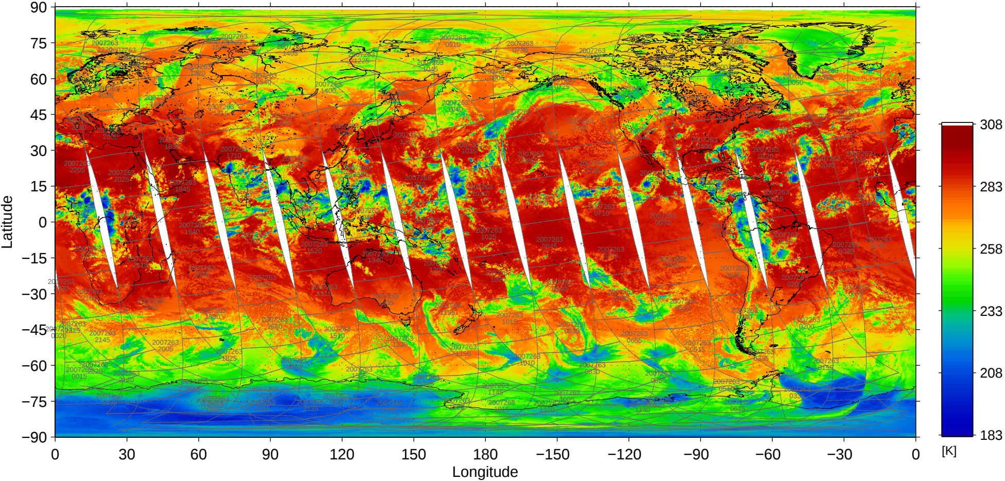
File = 200709/MOD02SSH-A2007263-pbin-005.1440-0721, band=31
