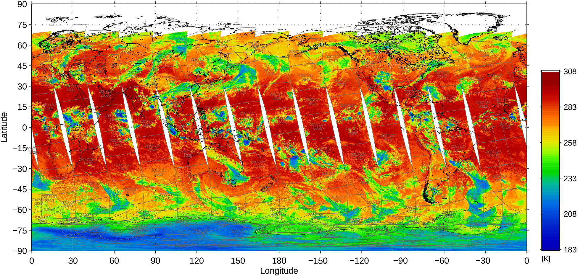
File = 200705/MOD02SSH-A2007137-pbin-005.1440-0721, band=31
