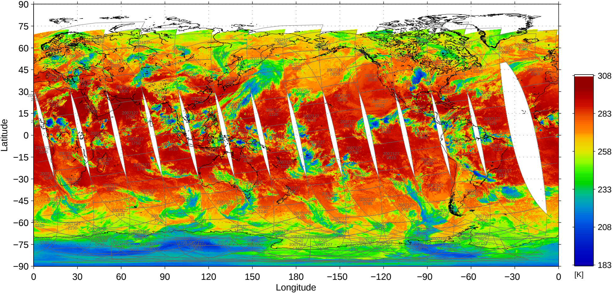
File = 200705/MOD02SSH-A2007127-pbin-005.1440-0721, band=31
