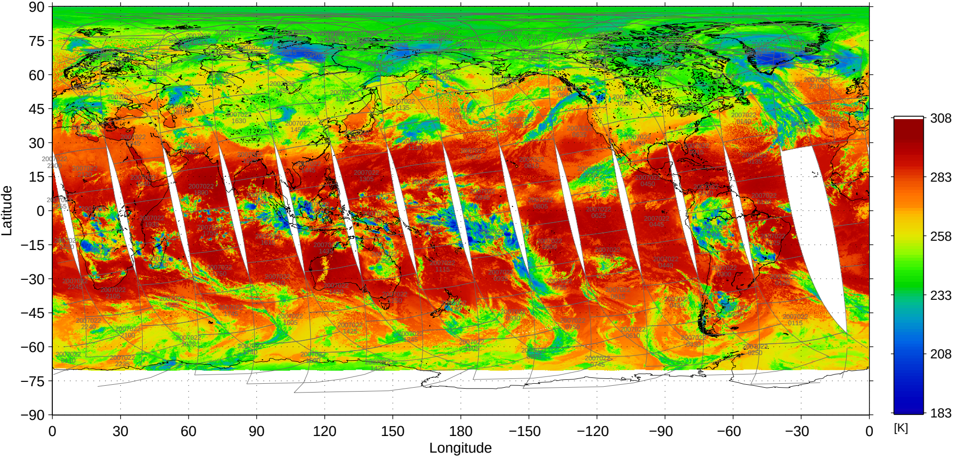
File = 200701/MOD02SSH-A2007022-pbin-005.1440-0721, band=31
