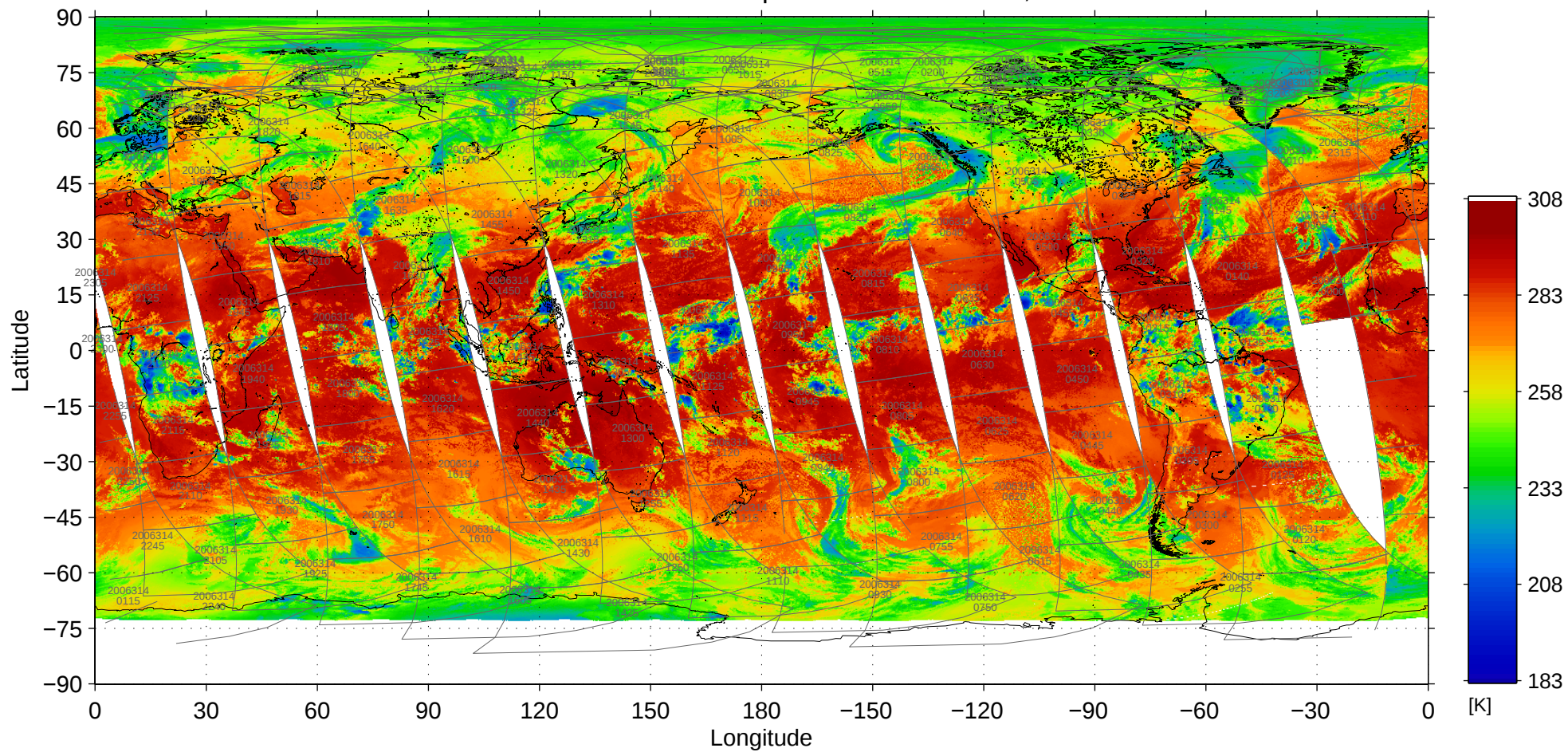
File = MOD02SSH-A2006314-pbin-005.1440-0721, band=31
