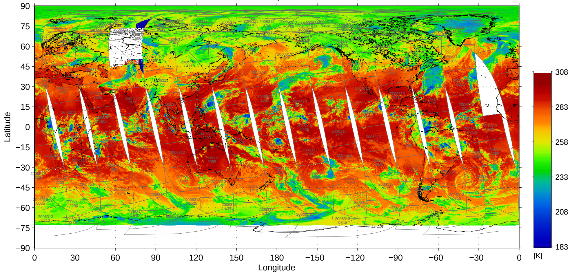
File = MOD02SSH-A2006313-pbin-005.1440-0721, band=31
