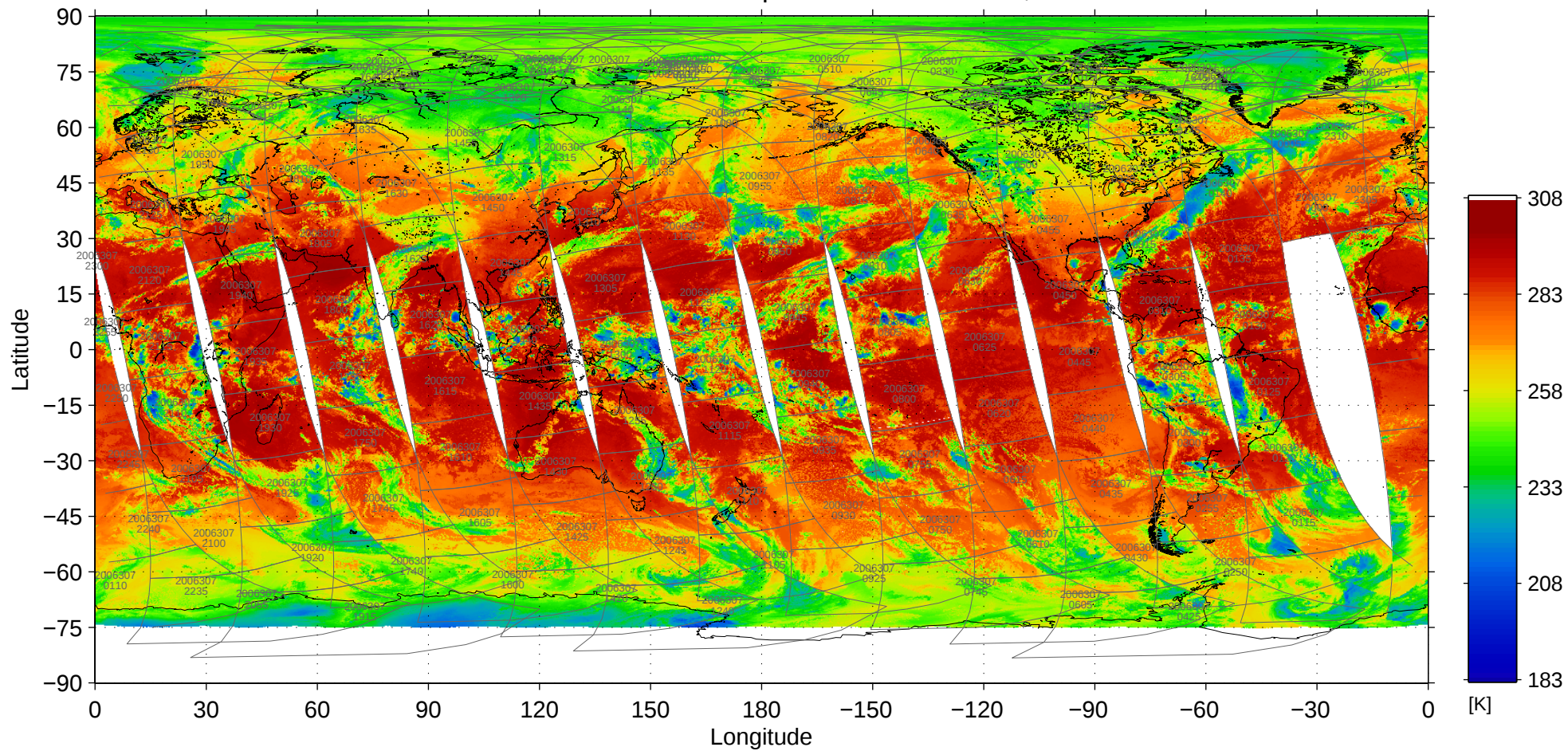
File = MOD02SSH-A2006307-pbin-005.1440-0721, band=31
