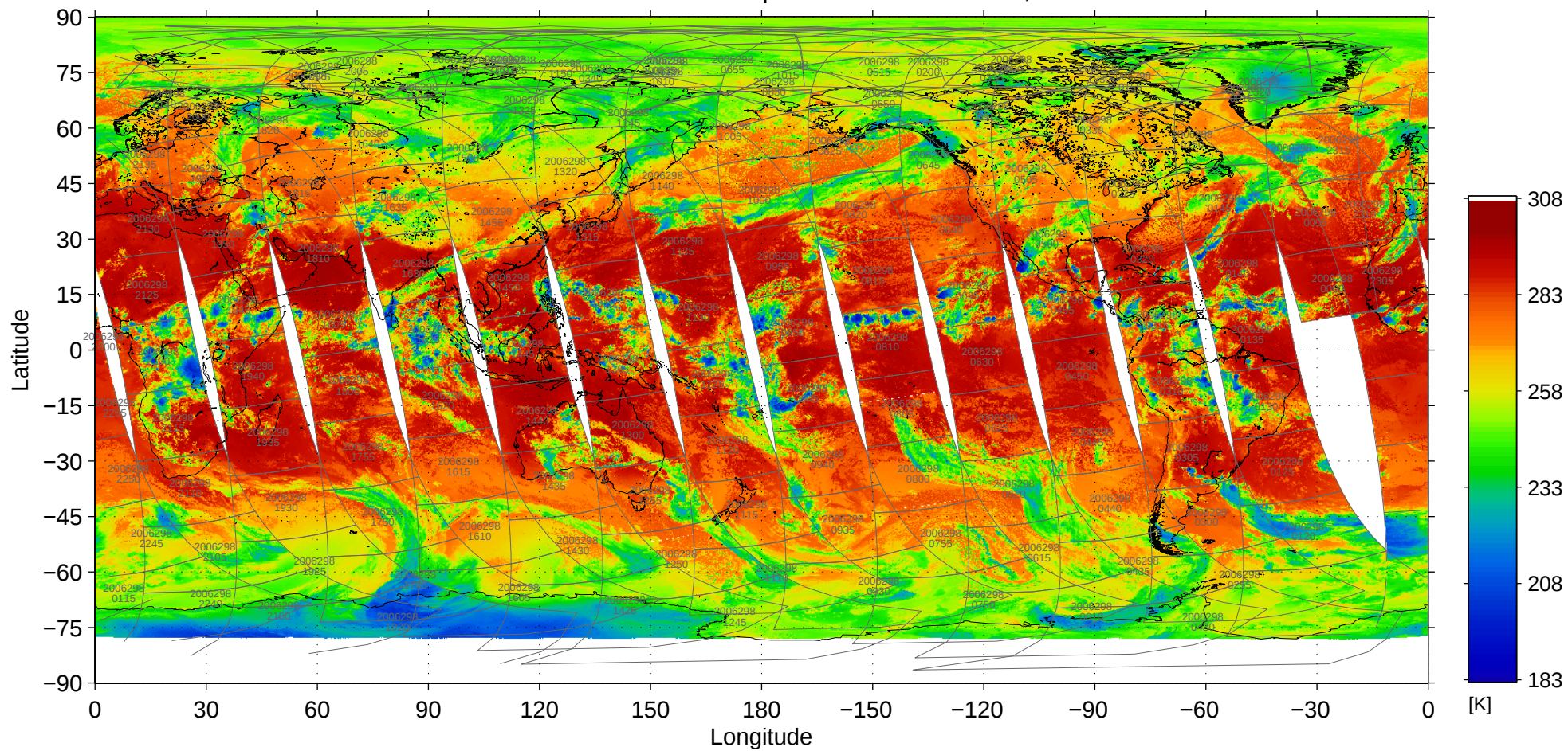
File = MOD02SSH-A2006298-pbin-005.1440-0721, band=31
