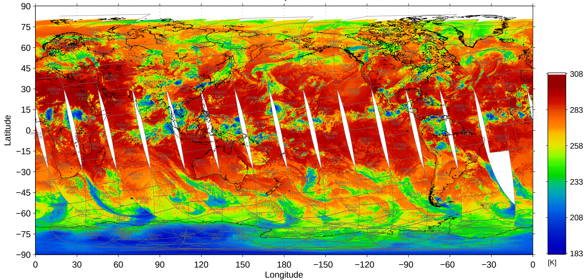
File = MOD02SSH-A2006241-pbin-005.1440-0721, band=31
