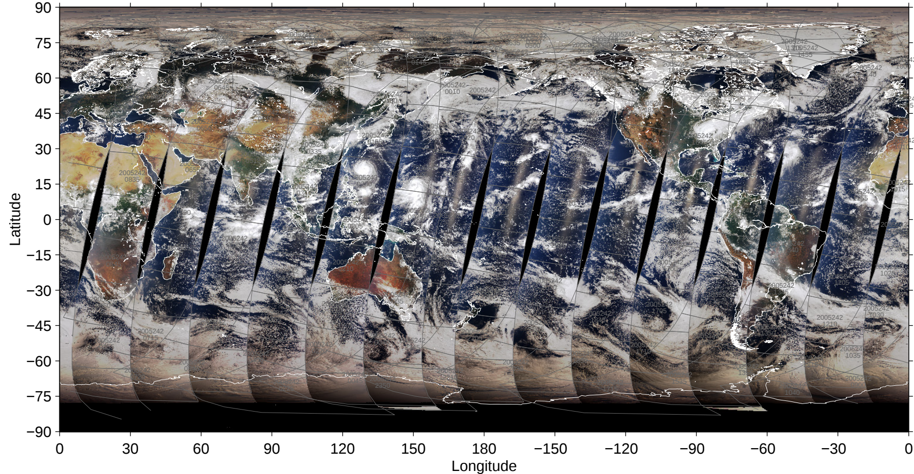
File = glmap-modis/MOD02SSH-A2005242-pbin-005.1440-0721, RGB=645, 555, 469nm
