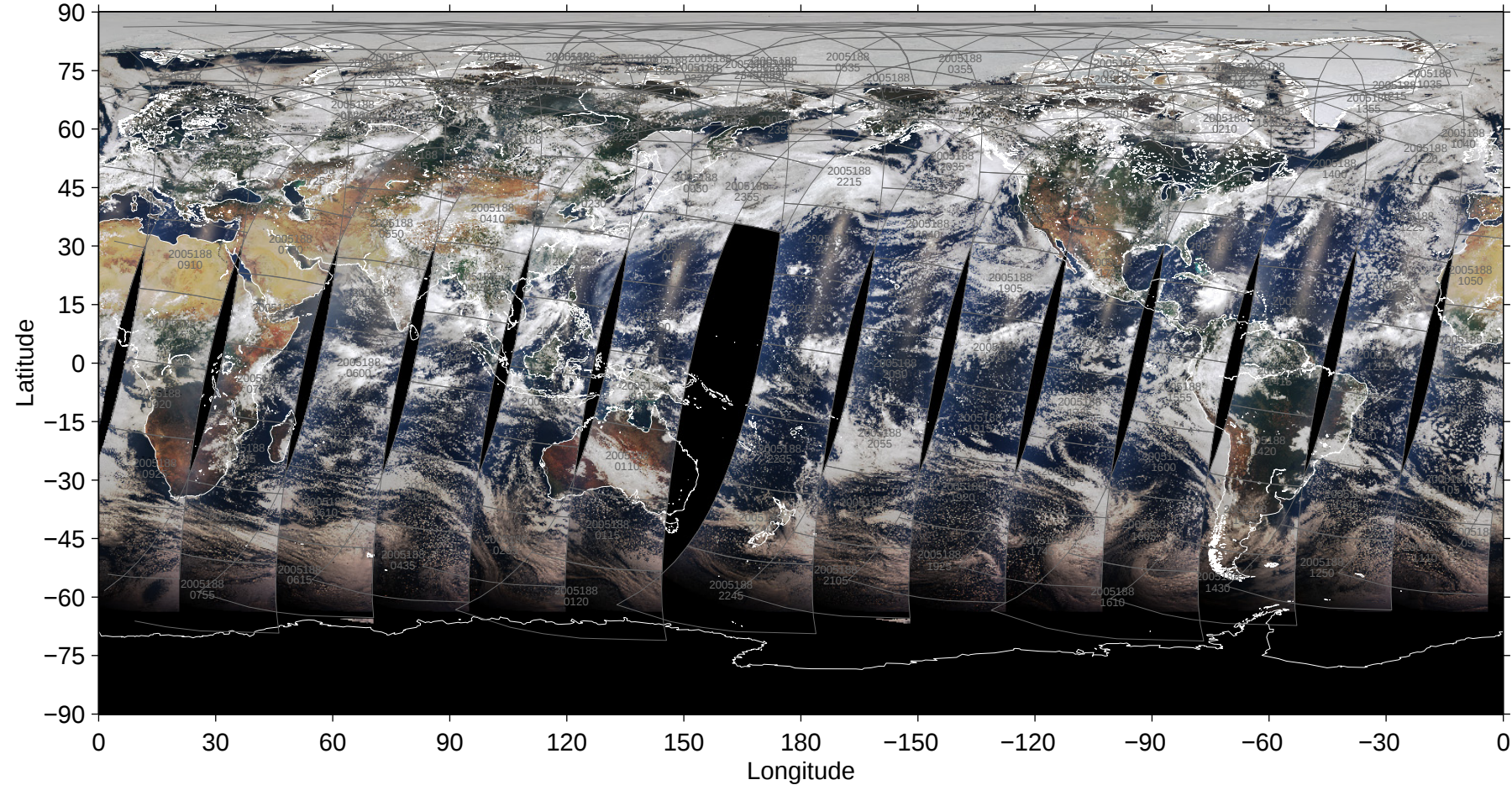
File = glmap-modis/MOD02SSH-A2005188-pbin-005.1440-0721, RGB=645, 555, 469nm
