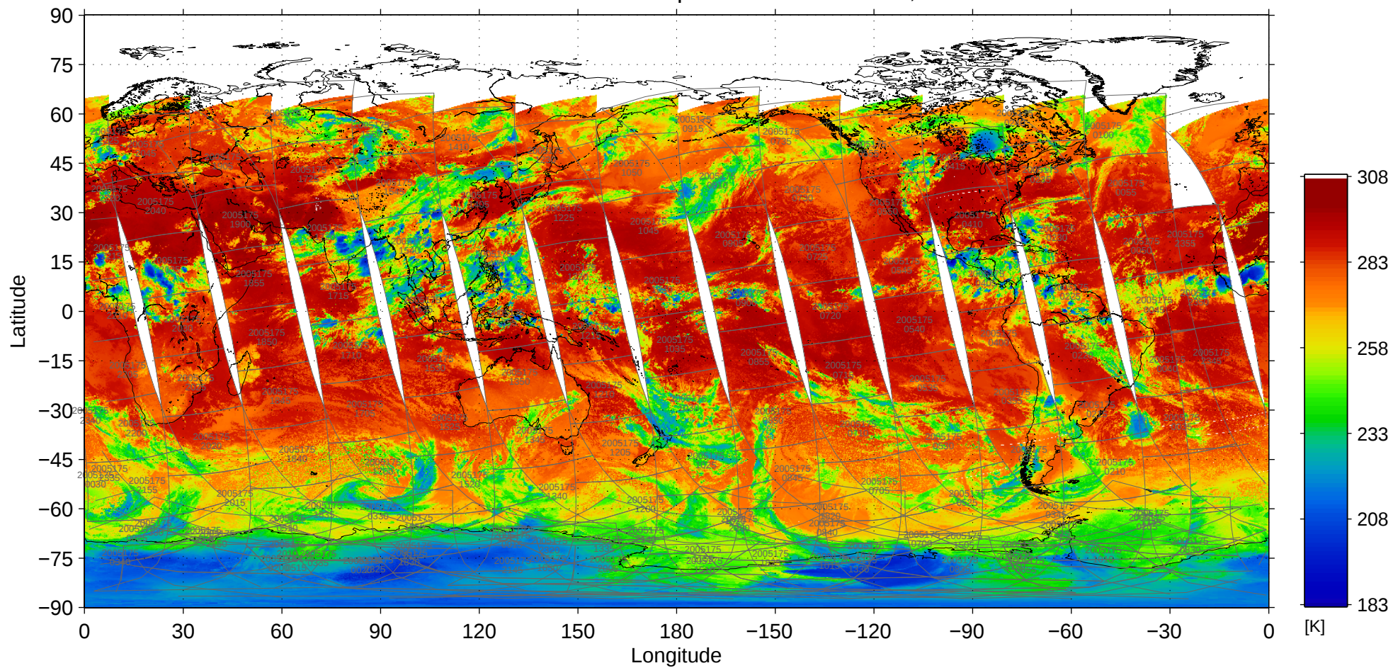
File = MOD02SSH-A2005175-pbin-005.1440-0721, band=31
