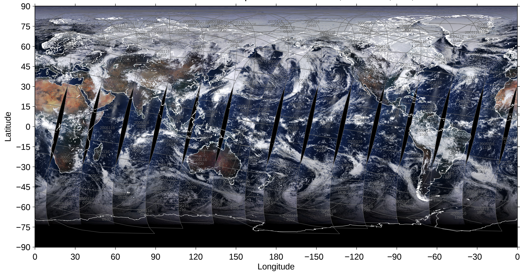
File = MOD02SSH-A2005116-pbin-005.1440-0721, RGB=645, 555, 469nm
