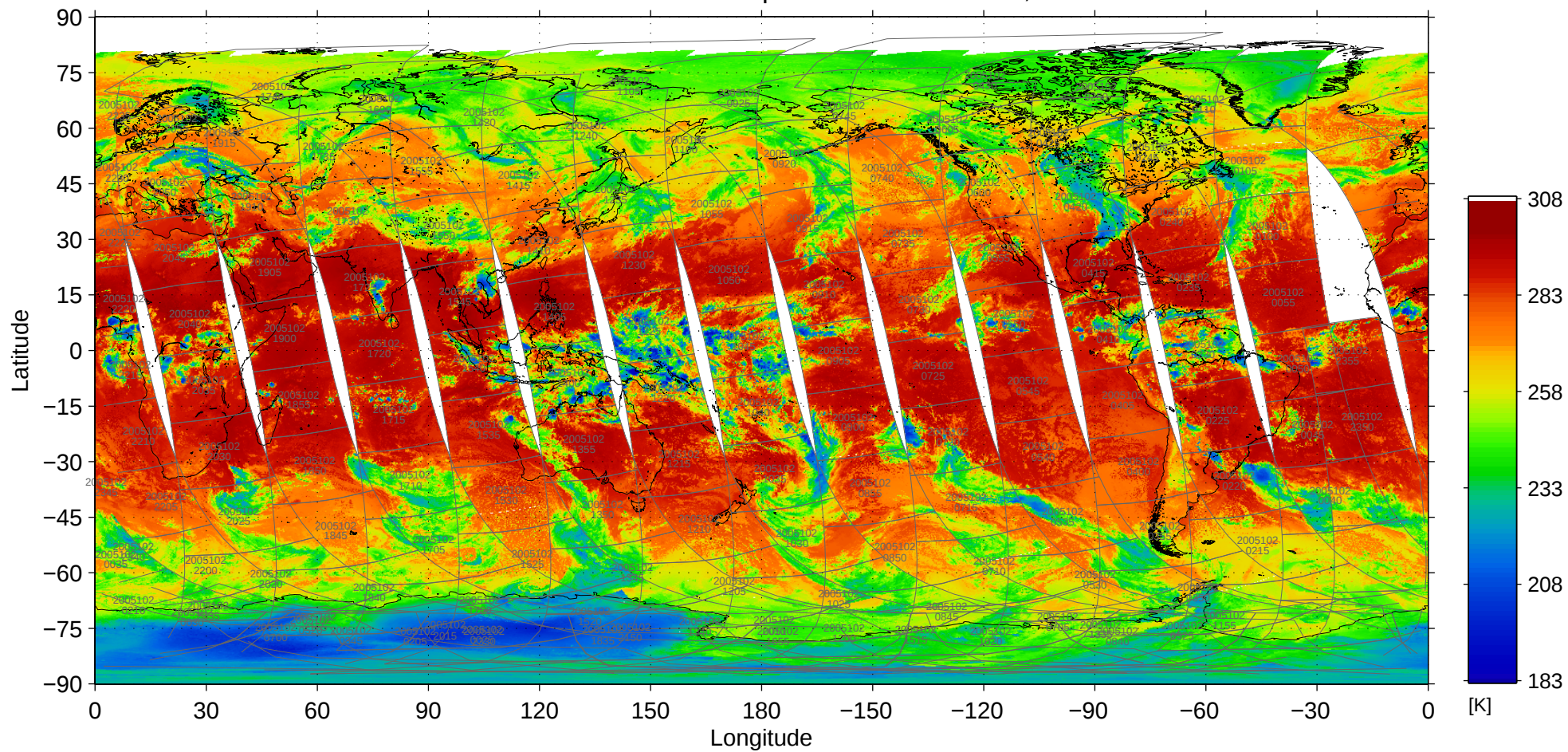
File = MOD02SSH-A2005102-pbin-004.1440-0721, band=31
