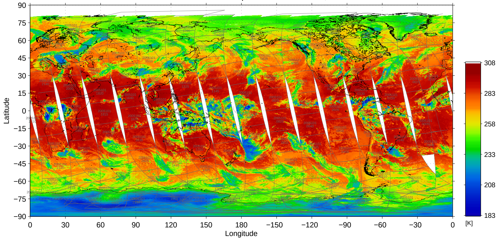
File = MOD02SSH-A2005101-pbin-004.1440-0721, band=31
