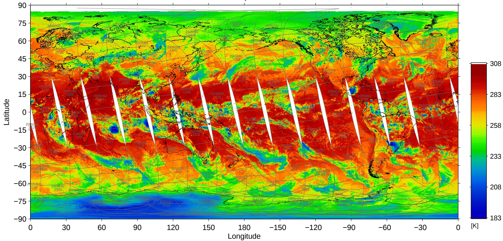
File = MOD02SSH-A2005092-pbin-004.1440-0721, band=31
