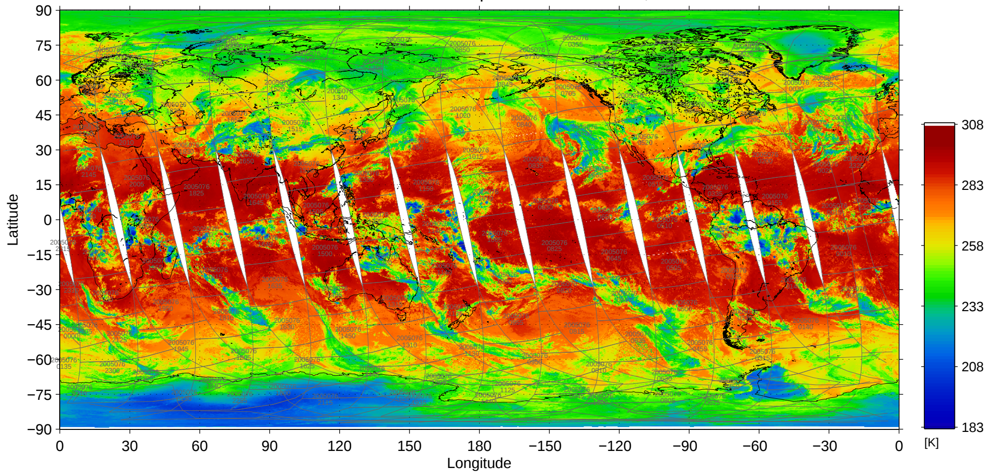
File = MOD02SSH-A2005076-pbin-004.1440-0721, band=31
