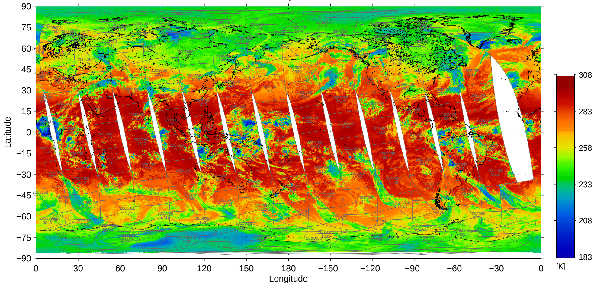
File = MOD02SSH-A2005068-pbin-004.1440-0721, band=31
