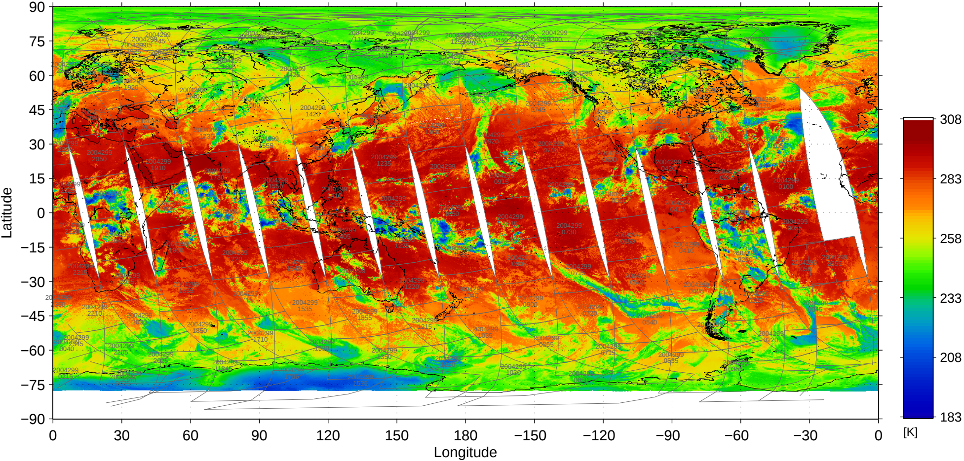
File = 200410/MOD02SSH-A2004299-pbin-004.1440-0721, band=31
