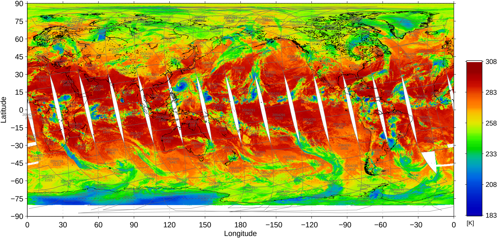
File = 200410/MOD02SSH-A2004291-pbin-004.1440-0721, band=31
