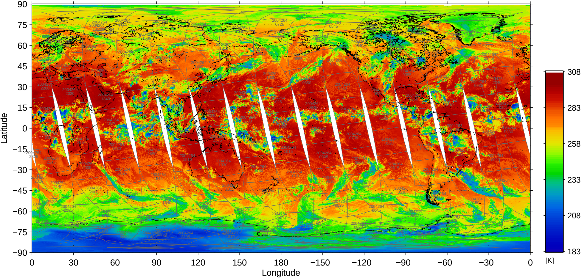
File = 200409/MOD02SSH-A2004264-pbin-004.1440-0721, band=31
