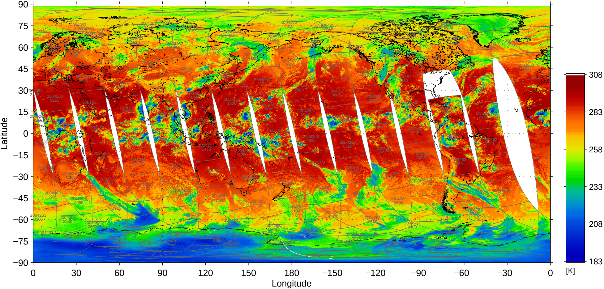
File = 200409/MOD02SSH-A2004263-pbin-004.1440-0721, band=31
