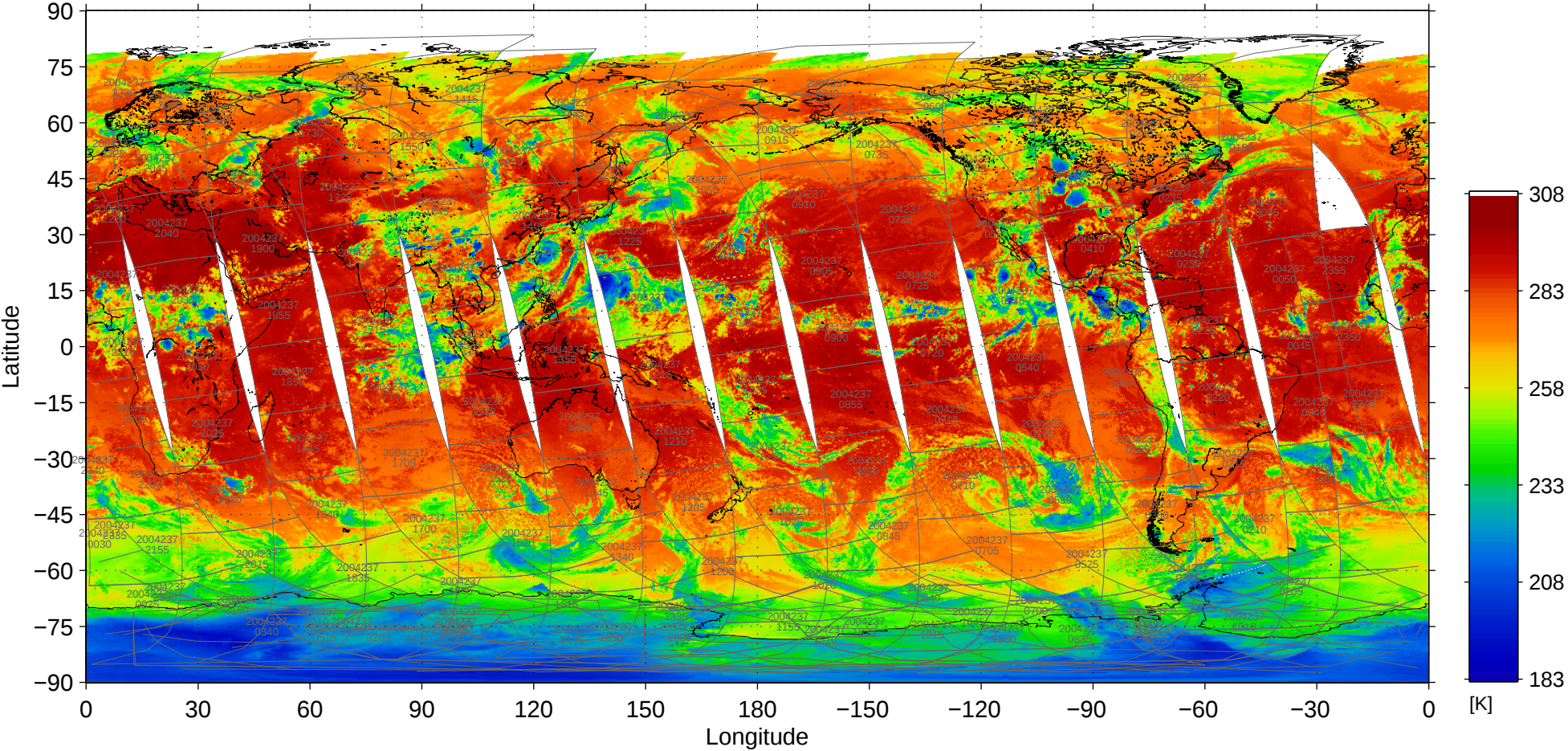
File = 200408/MOD02SSH-A2004237-pbin-004.1440-0721, band=31
