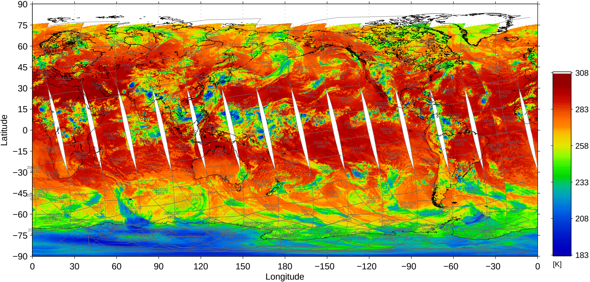
File = 200408/MOD02SSH-A2004230-pbin-004.1440-0721, band=31
