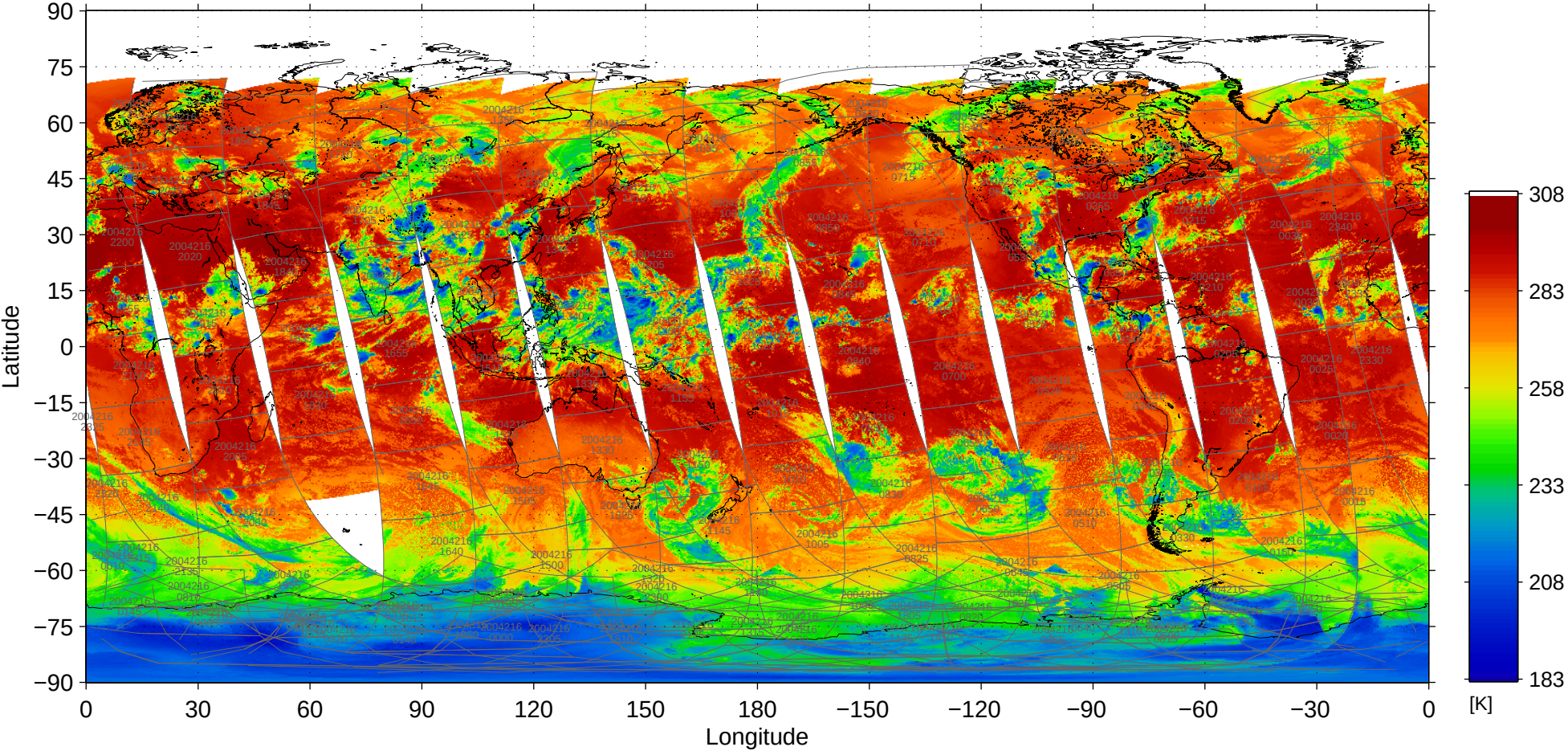
File = 200408/MOD02SSH-A2004216-pbin-004.1440-0721, band=31
