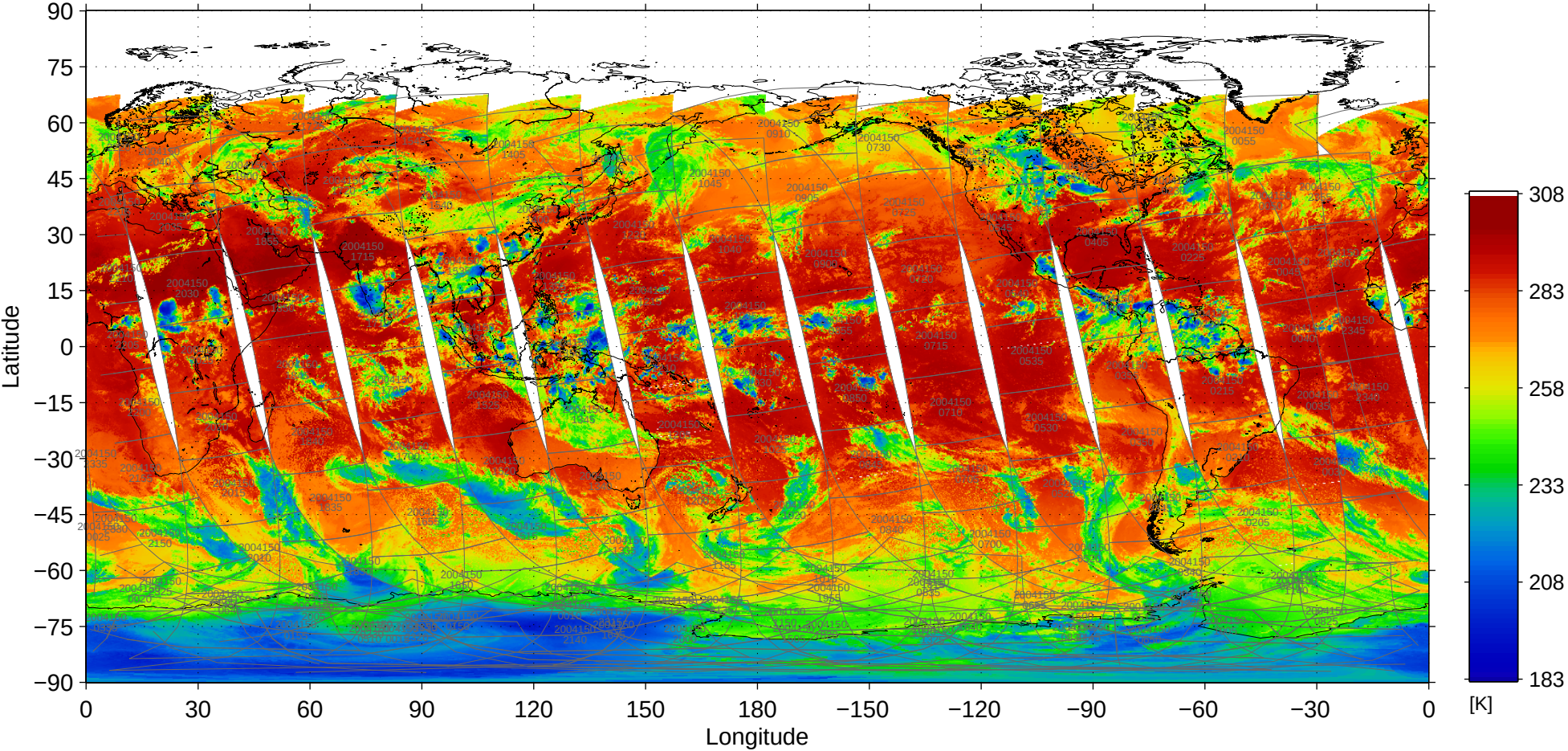
File = 200405/MOD02SSH-A2004150-pbin-004.1440-0721, band=31
