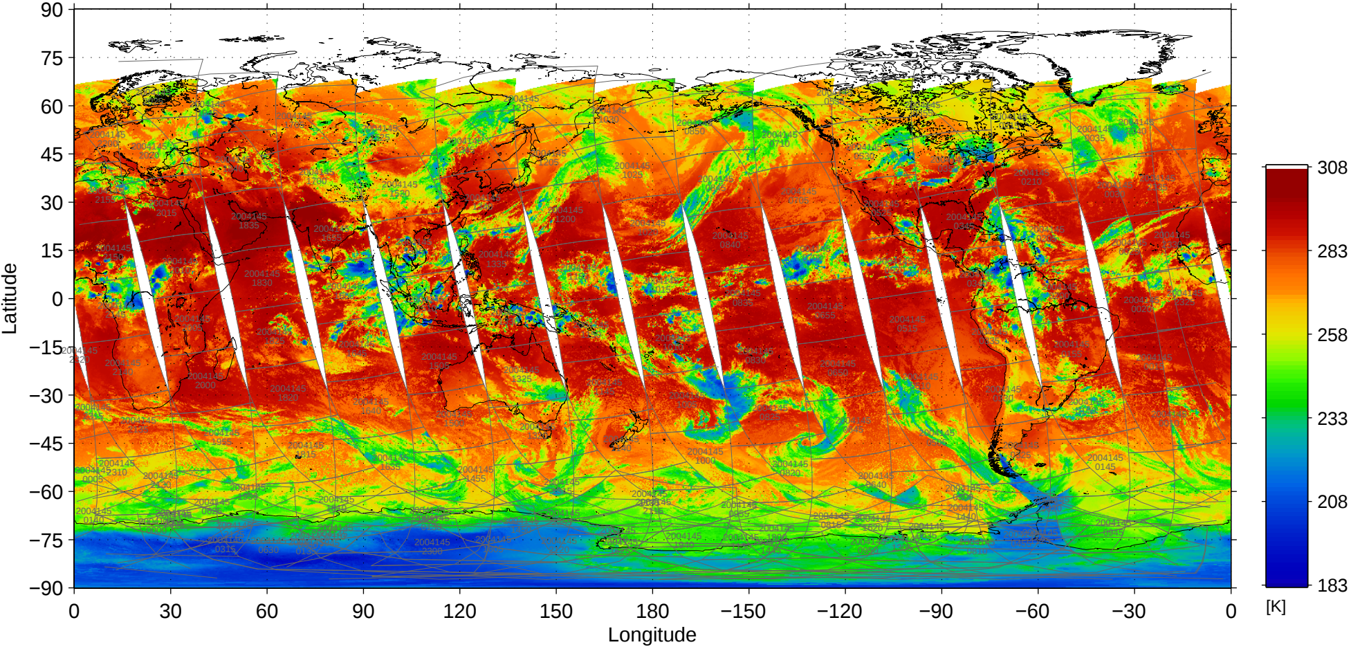
File = 200405/MOD02SSH-A2004145-pbin-004.1440-0721, band=31
