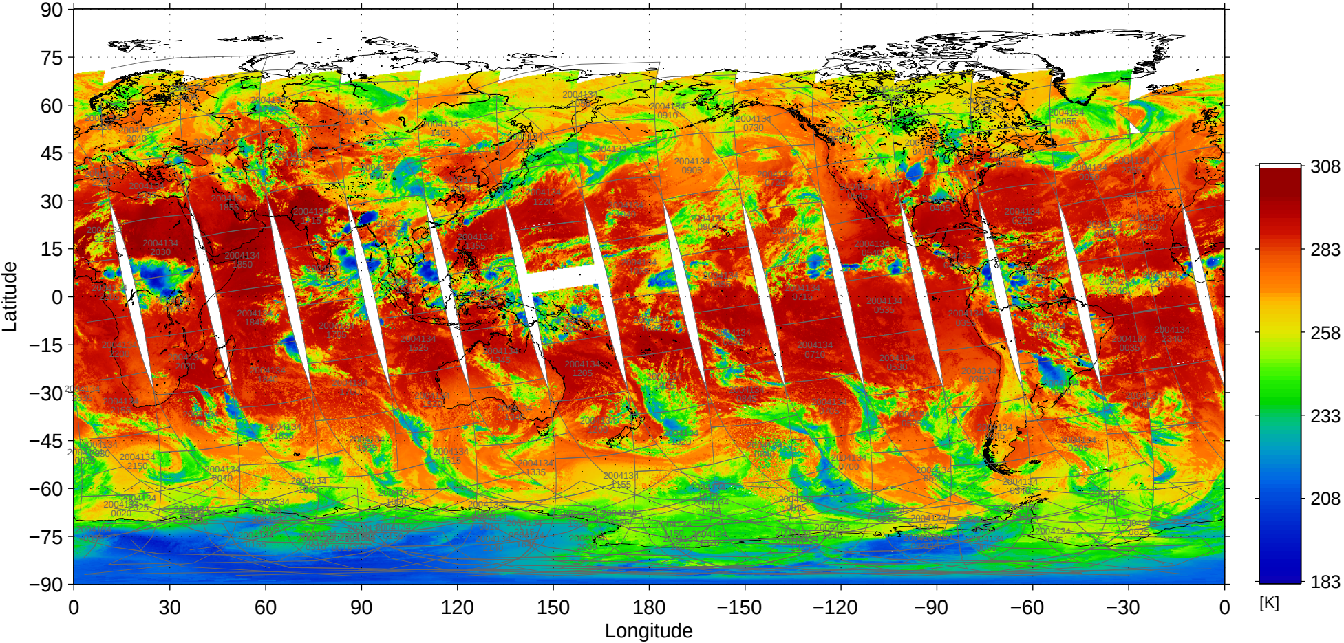
File = 200405/MOD02SSH-A2004134-pbin-004.1440-0721, band=31
