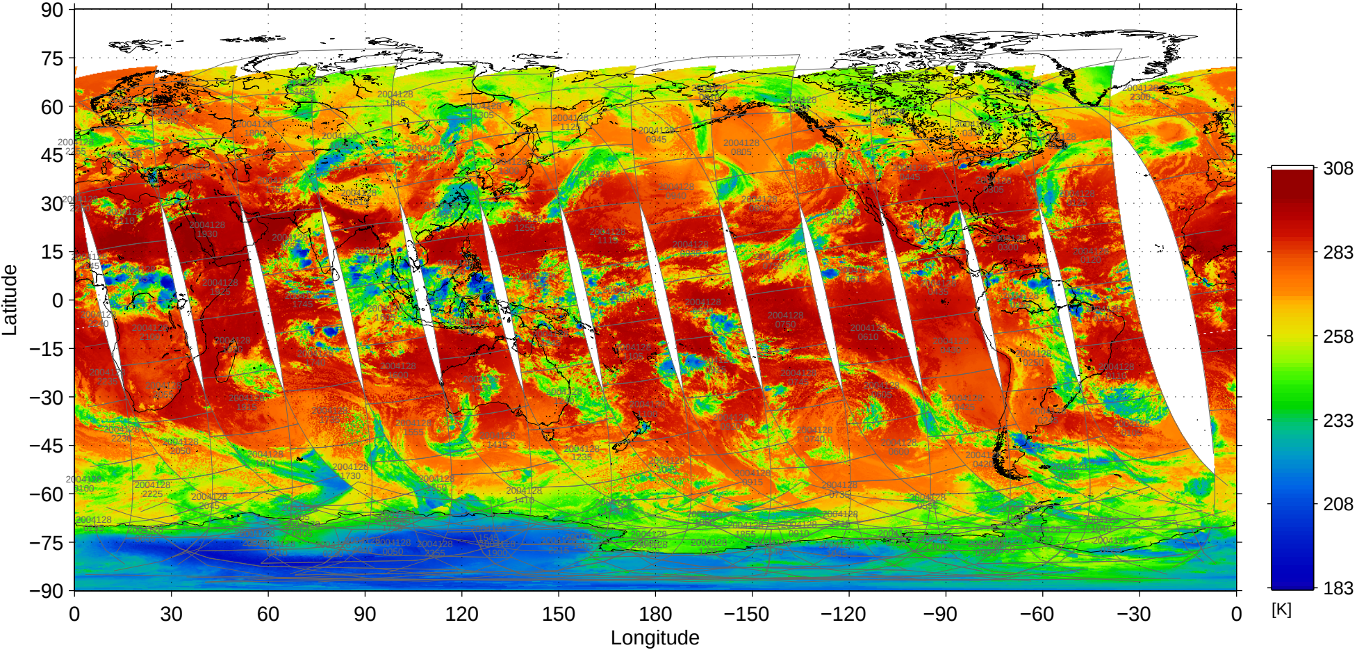
File = 200405/MOD02SSH-A2004128-pbin-004.1440-0721, band=31
