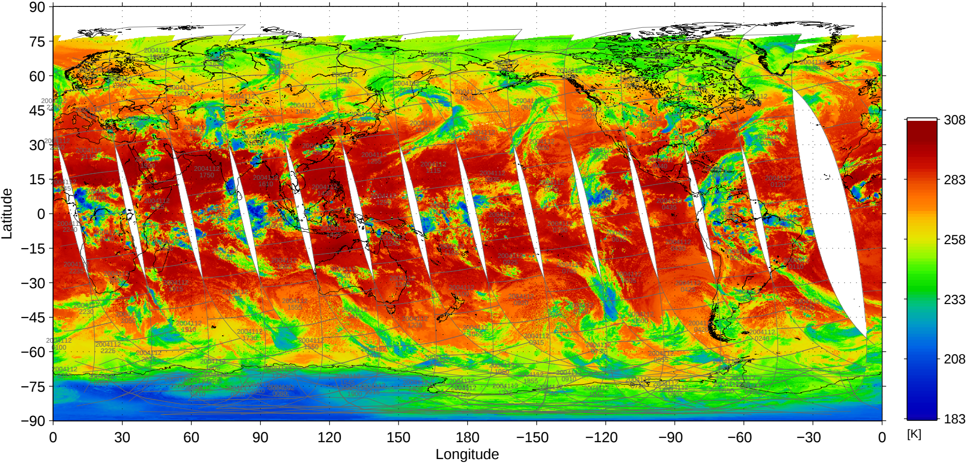
File = 200404/MOD02SSH-A2004112-pbin-004.1440-0721, band=31
