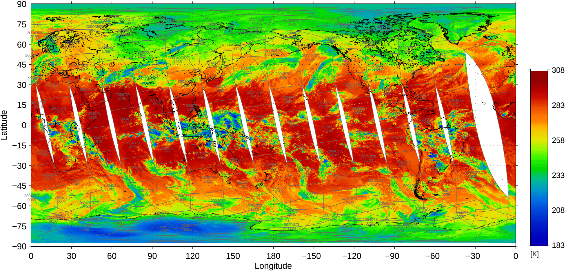
File = 200403/MOD02SSH-A2004073-pbin-004.1440-0721, band=31
