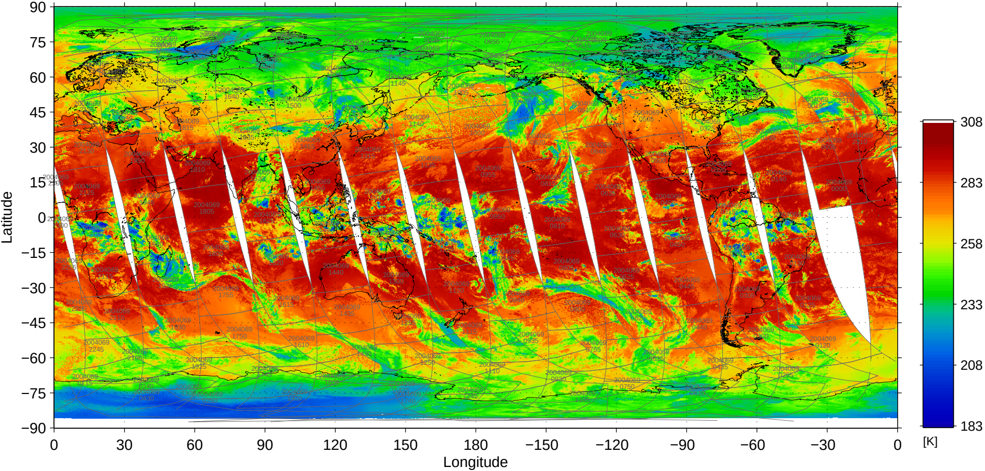
File = 200403/MOD02SSH-A2004069-pbin-004.1440-0721, band=31
