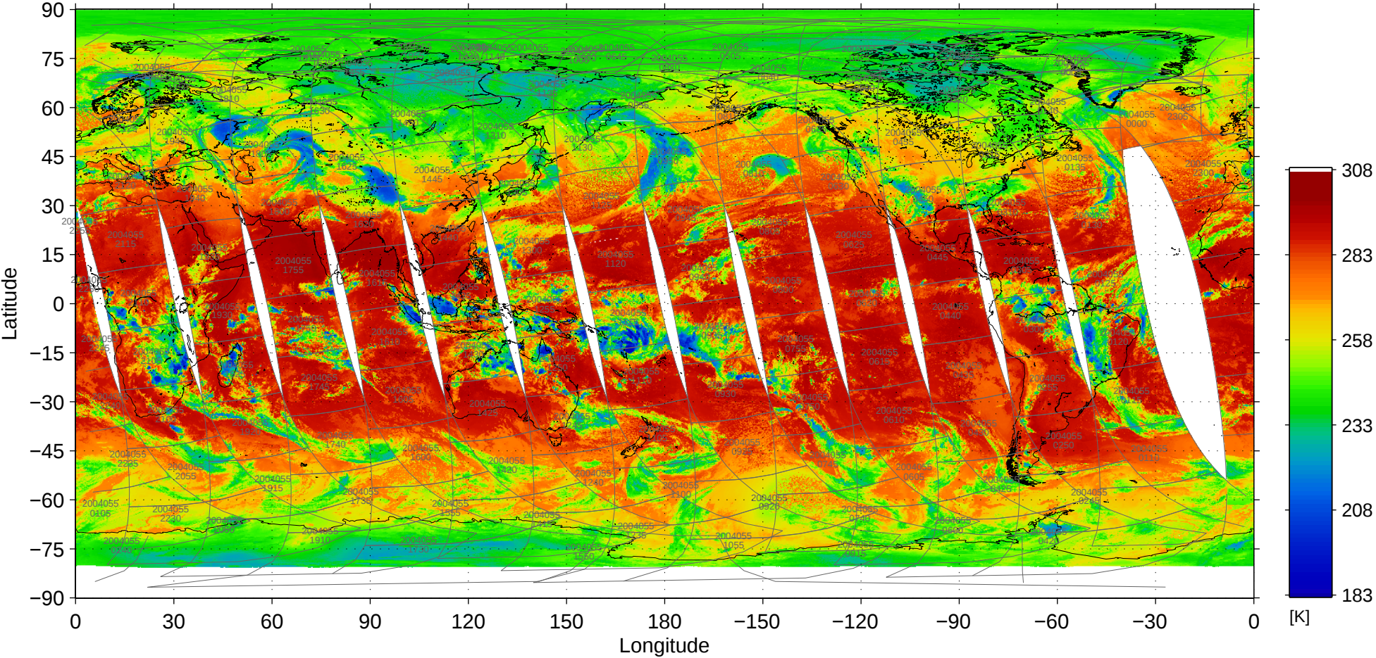
File = 200402/MOD02SSH-A2004055-pbin-004.1440-0721, band=31
